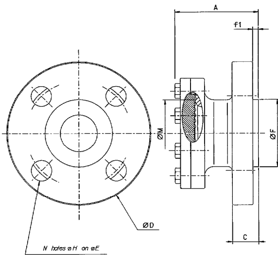
Flange adaptor
